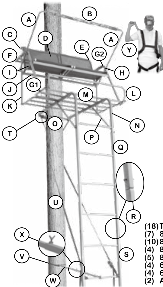
FIGURE 1: RHINO TREESTANDS RTL-4000 COMPONENTS
