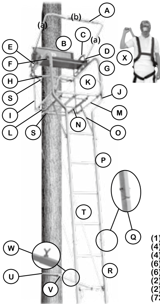
FIGURE 1: RHINO TREESTANDS RTL-300 COMPONENTS
