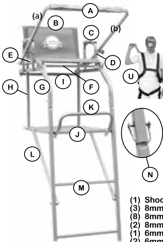
FIGURE 1: RHINO TREESTANDS RTL-200 COMPONENTS
